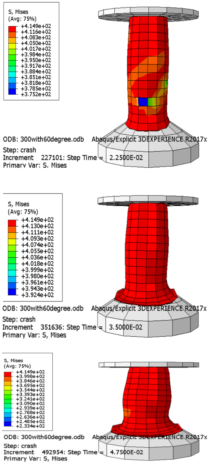
Figure 12: Modeling deformation of Second rail
