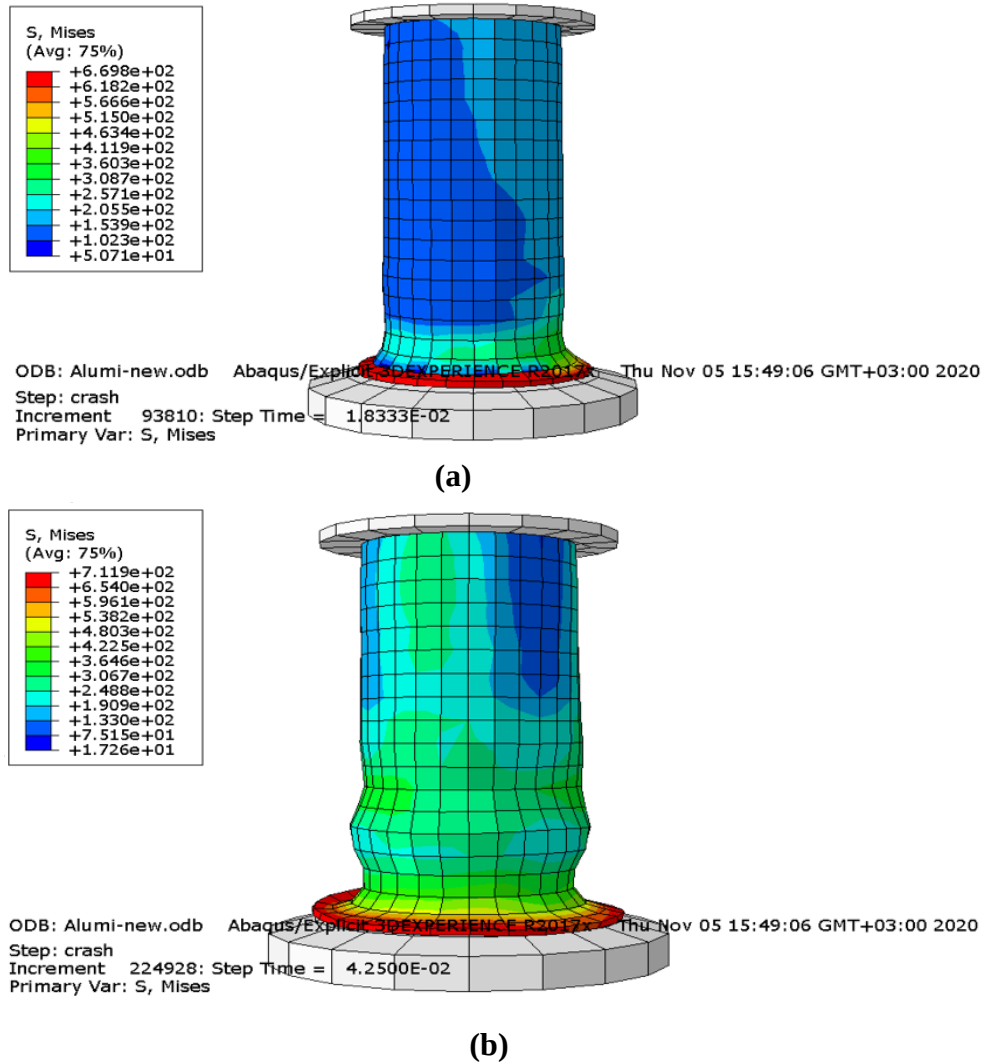
Figure 9: Modeling deformation of first trail
