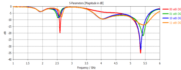
Fig. 7; S_{11} parameter of the proposal design with DGS and length of ground equal 25mm.
