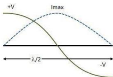
Fig. 2: Current and voltage variation.
