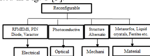
Fig. 1; Antenna reconfiguration techniques.
