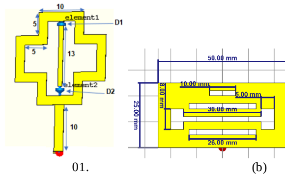
Fig. 3; Proposed Antenna Design: (a) Front view:consisting of patch dimension and (b) Back view (ground plane): including the height of the ground plane with DGS.
