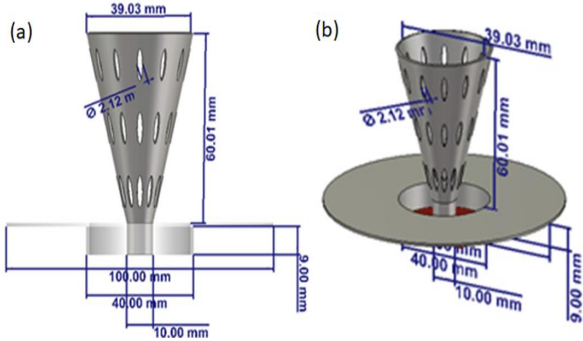
Fig. 4; The proposed sensor based on 3D antenna geometry: (a) Front view and (b) 3D view.
