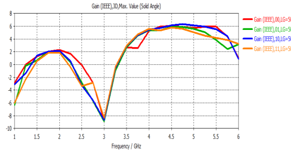
Fig. 11; Antenna gain spectra with DGS and length of ground=50mm.
