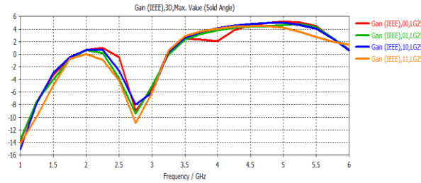
Fig. 10; Antenna gain spectra with DGS and length of ground=25mm.
