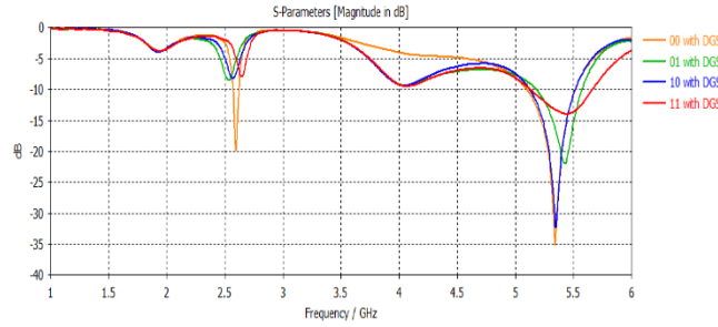
Fig. 6; S_{11} parameter of the proposal design.
