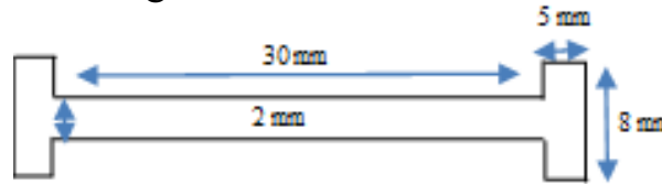
Fig. 4; Dumbbell shaped DGS with dimensions.
