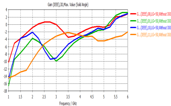
Fig. 12; Antenna gain spectra without DGS and length of ground=50mm.
