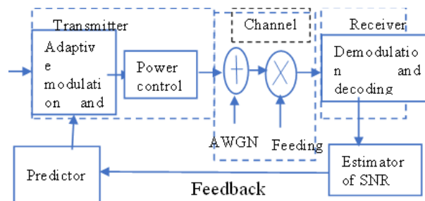
Fig. 5; Typical adaptive modulation system.
