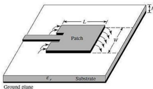
Fig. 1: A microstrip antenna structure.
