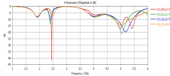
Fig. 8; S_{11} parameter of the proposal design with DGS and length of ground equal 50mm.
