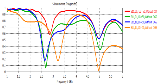
Fig. 9; S_{11} parameter of the proposal design without DGS and length of ground equal 50mm.
