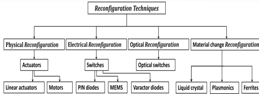
Fig. 4; Reconfiguration techniques of reconfigurable antennas.
